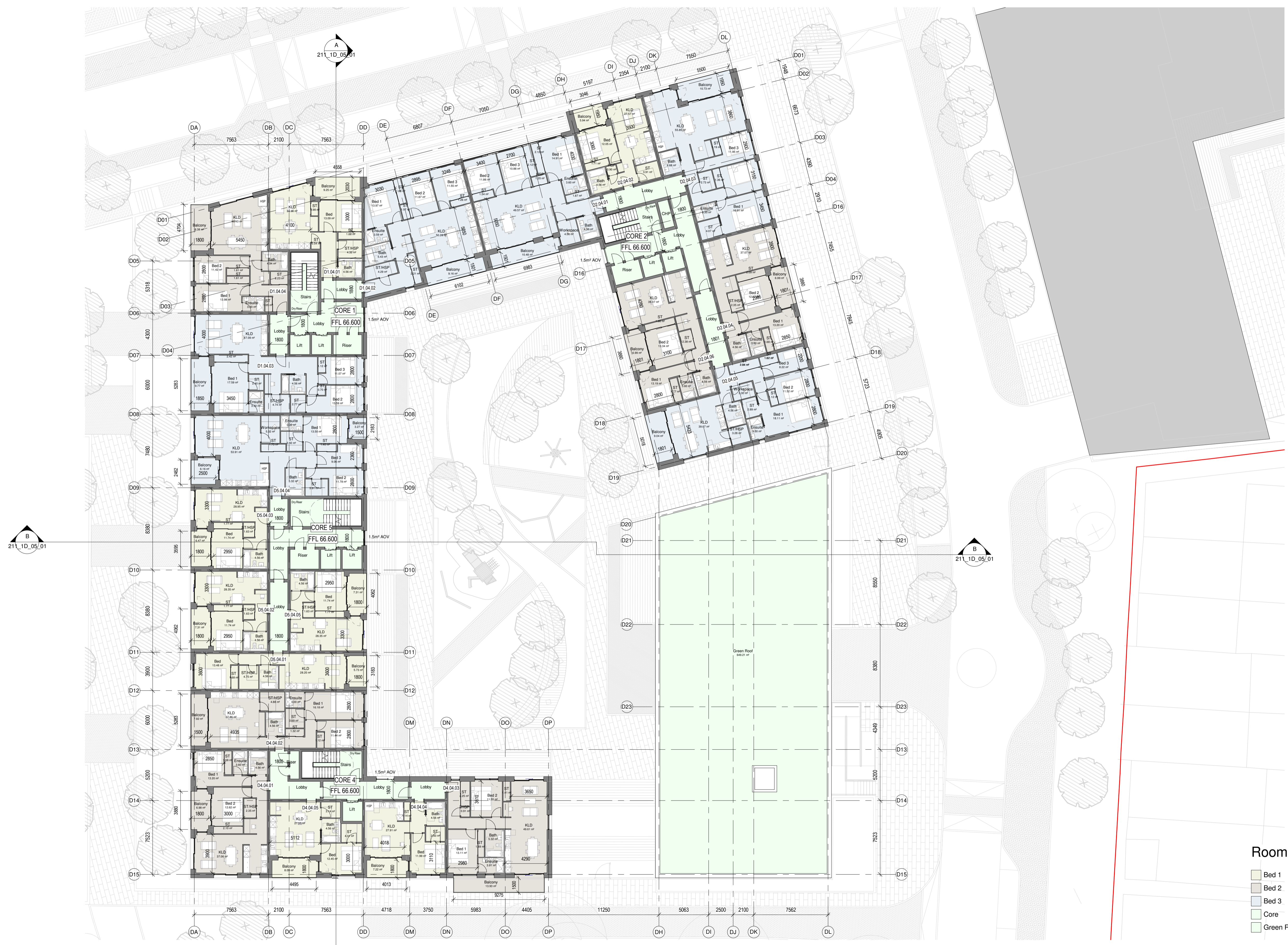
1 Block 1D_Fourth Floor Plan 1 : 200
