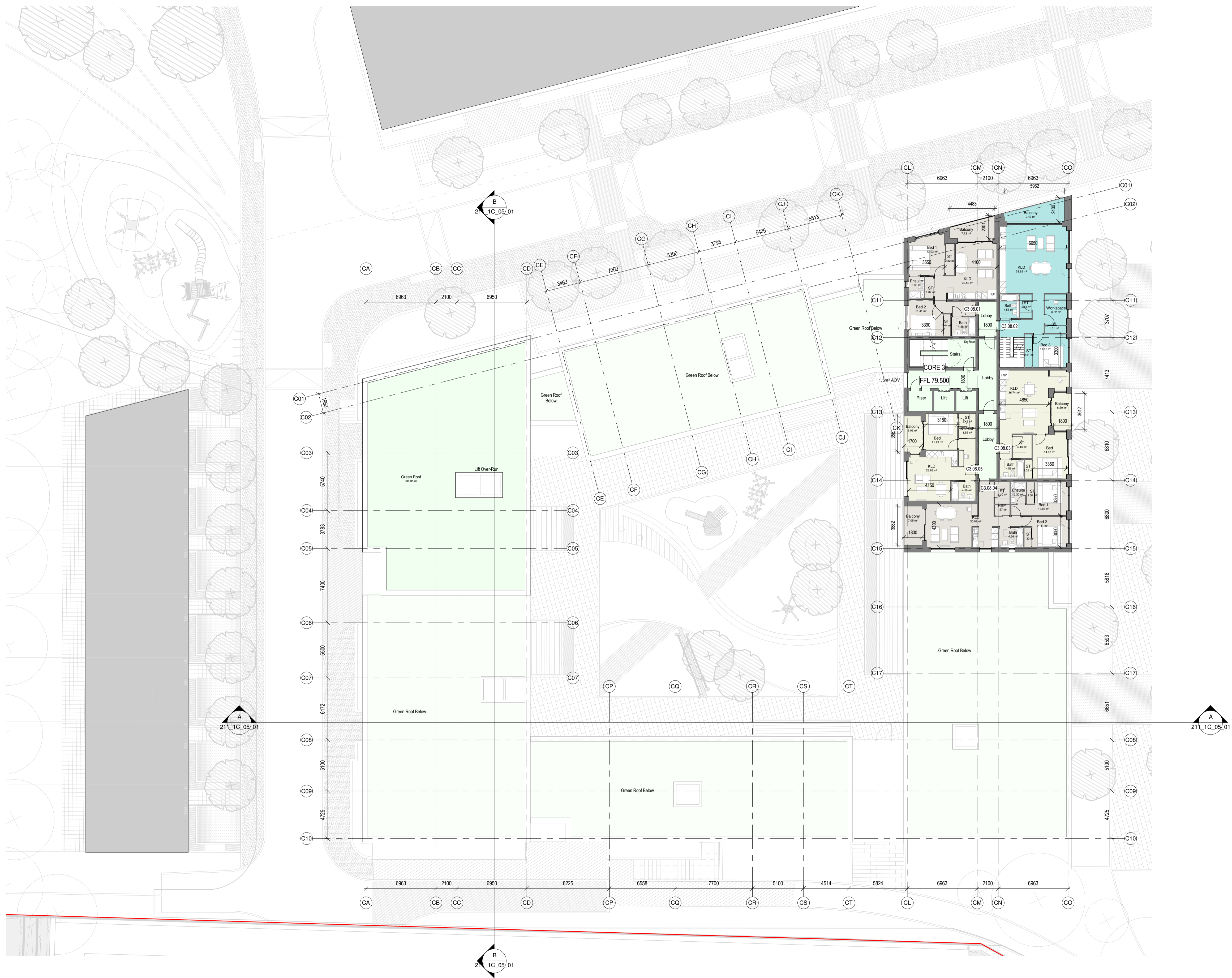
Block 1C_Eighth Floor Plan 1 : 200
